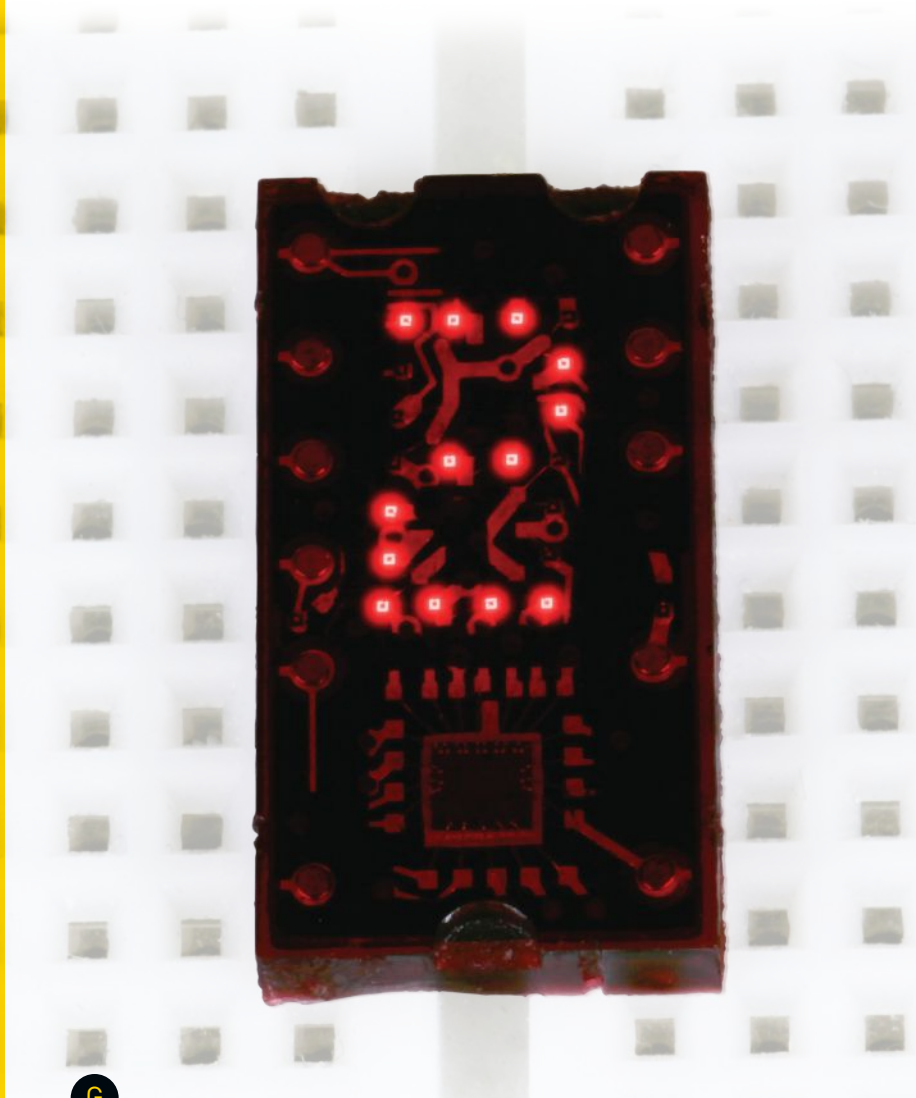
Texas Instruments TIL311. 5VDC. Total supply current for logic plus LEDs: typically about 100mA.
