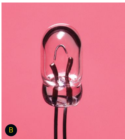
JKL Lamps #683. 5V, 60mA, rated 100,000 hours.
